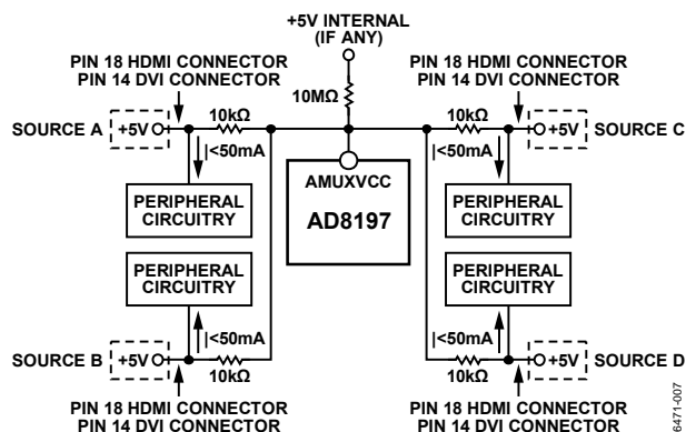
Figure 28. Suggested AMUXVCC Power Scheme
