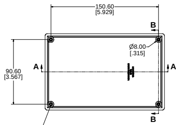
TOP VIEW OF BOX
