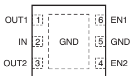
TPS718xx, TPS719xx DRV Package 2mm x 2mm SON-6 (Top View)
