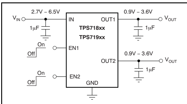
Figure 22. Typical Application Circuit
