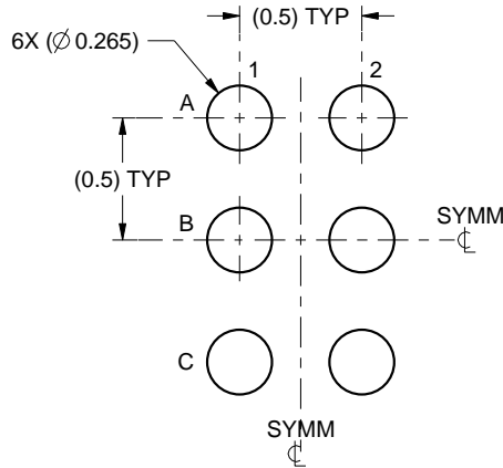
LAND PATTERN EXAMPLE SCALE:30X
