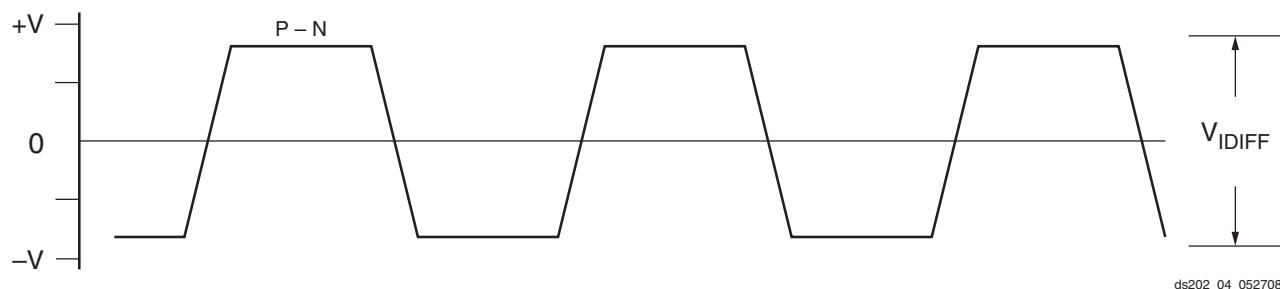
Figure 4: Differential Clock Input Voltage Swing Peak-to-Peak
