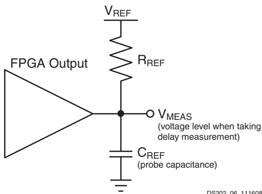
Figure 11: Single Ended Test Setup
