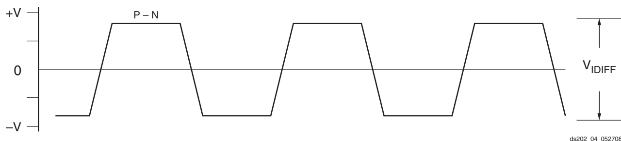
Figure 9: Differential Clock Input Voltage Swing Peak-to-Peak
