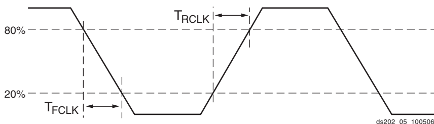
Figure 10: Reference Clock Timing Parameters
