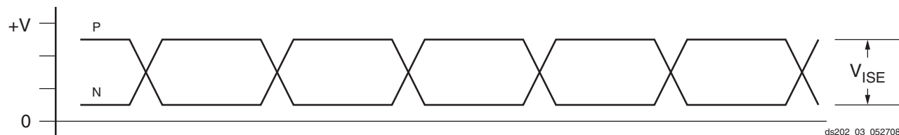
Figure 8: Single-Ended Clock Input Voltage Swing Peak-to-Peak
