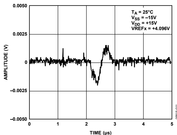
Figure 12. Digital Crosstalk
