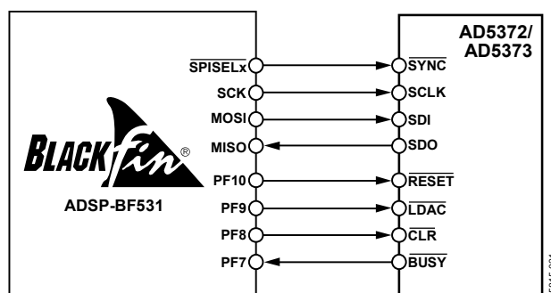
Figure 22. Interfacing to a Blackfin DSP
