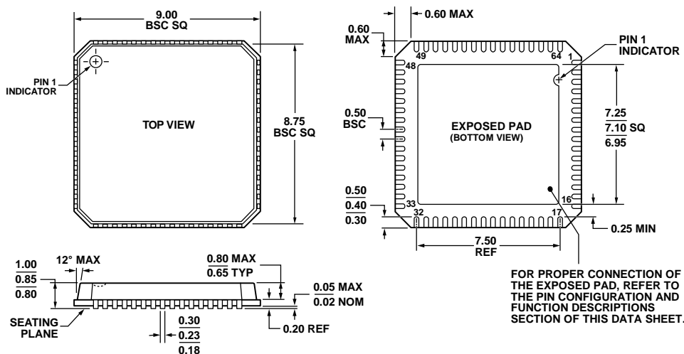
Figure 24. 64-Lead Lead Frame Chip Scale Package [LFCSP_VQ] 9 mm × 9 mm Body, Very Thin Quad (CP-64-3) Dimensions shown in millimeters
