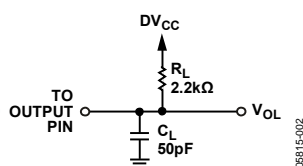
Figure 2. Load Circuit for \overline{BUSY} Timing Diagram
