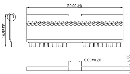
HM2SC22A8LF
