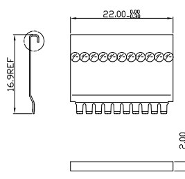
HM2SC11A8LF
