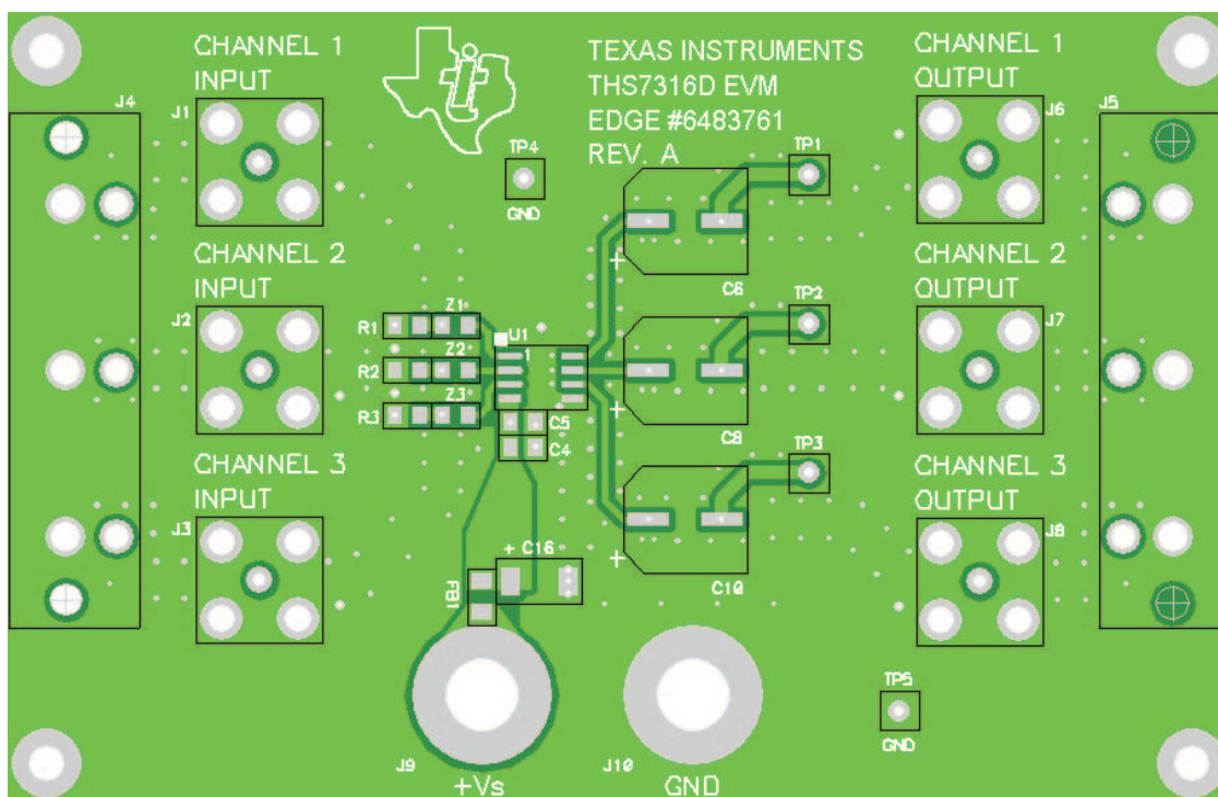
Figure 34. Top View
