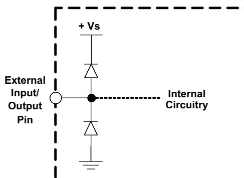
Figure 26. Internal ESD Protection
