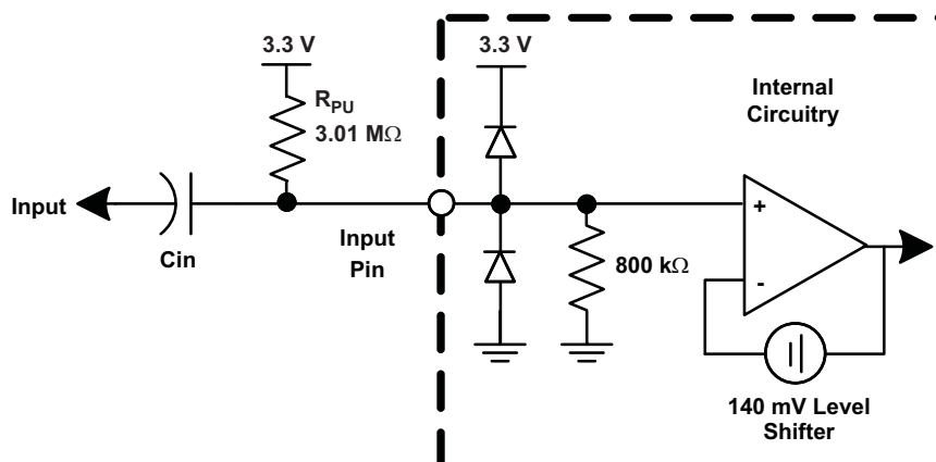
Figure 30. AC-Bias Input Mode Circuit Configuration
