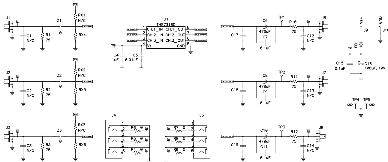
Figure 33. THS7316D EVM
