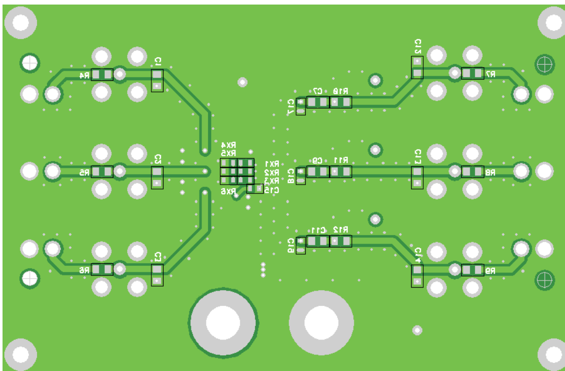
Figure 35. Bottom View
