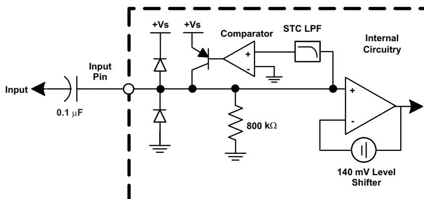
Figure 29. Equivalent AC Sync Tip Clamp Input Circuit
