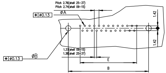
PC board drilling dimensions(after plating) (thickness ≤ 3.20±0.30mm)
