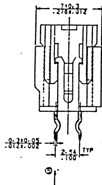
DETAIL T
