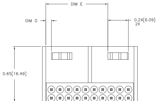
VIEW G-G
