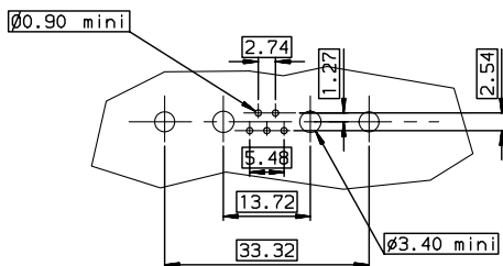
LAYOUT DIMENSIONS (after plating) CONNECTOR SIDE VIEW
