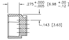
SECTION X-X
