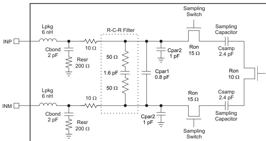
Figure 38. Input Stage
