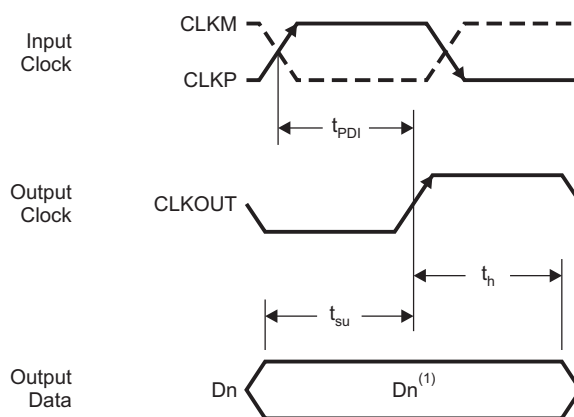
Figure 2. LVDS Mode Timing
