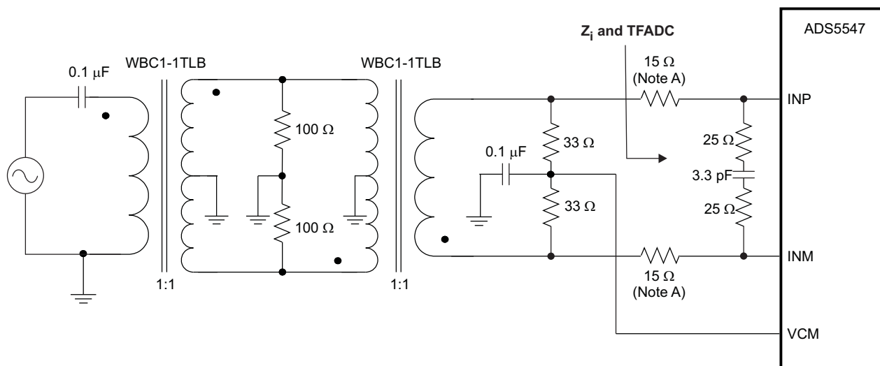
Figure 39. Example Drive Circuit With RF Transformers
