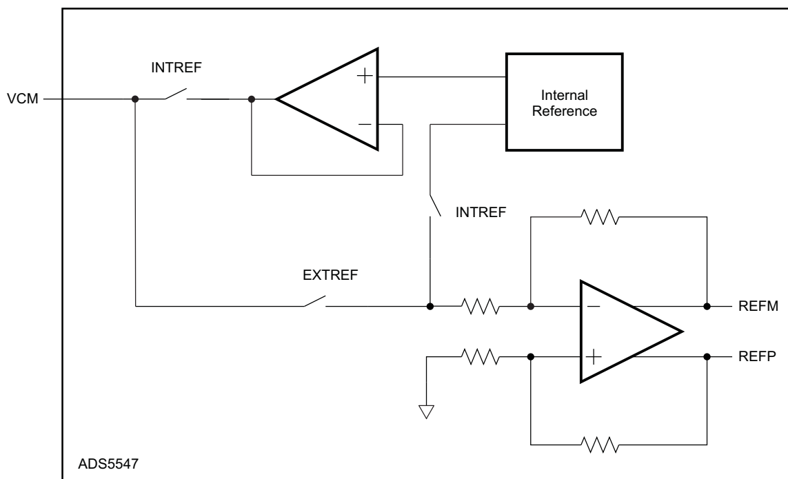
Figure 43. Reference Section
