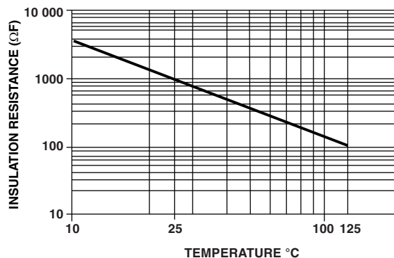
MINIMUM INSULATION RESISTANCE VS. TEMPERATURE
