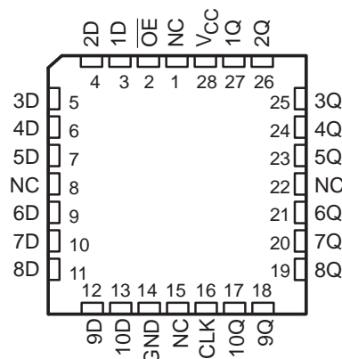
SN54AS821A . . . FK PACKAGE (TOP VIEW)
