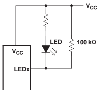
Figure 29. High-Value Resistor In Parallel With Led
