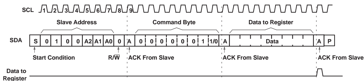
Figure 25. Write To Configuration Or Polarity Inversion Registers
