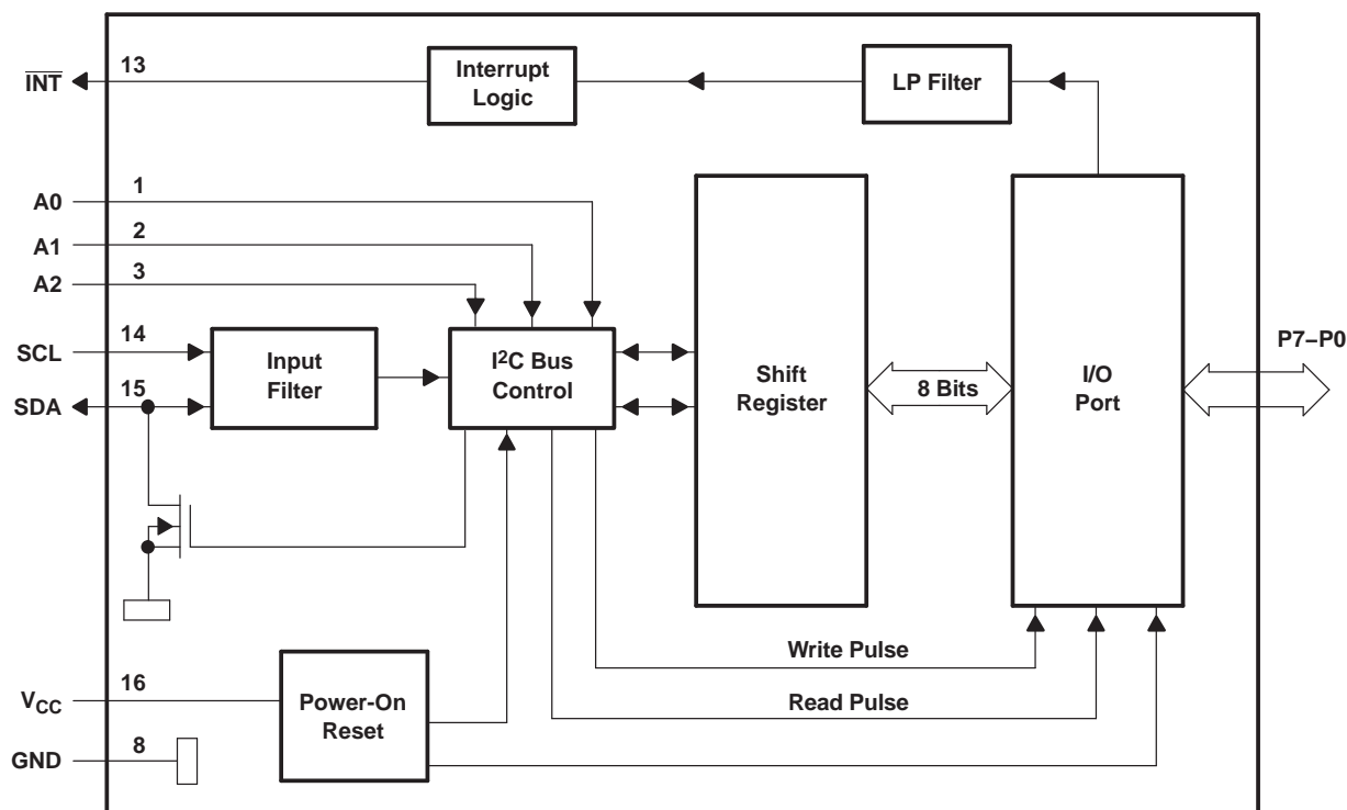
Figure 17. Logic Diagram
