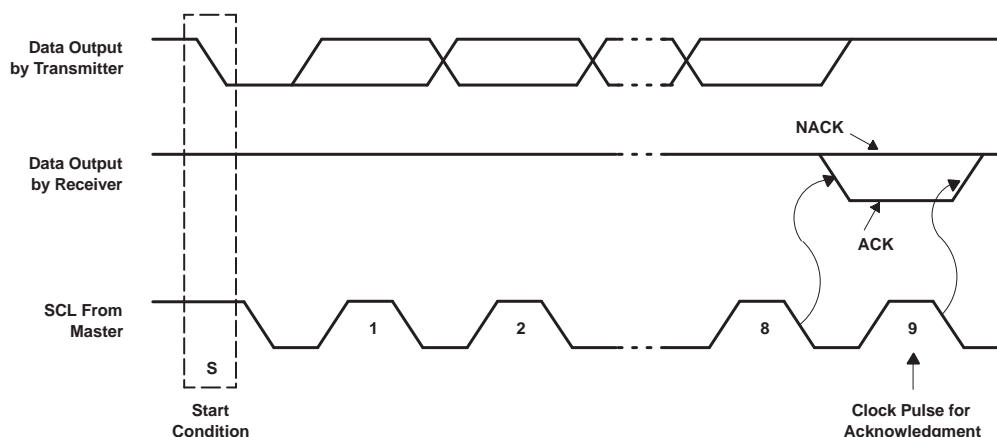
Figure 21. Acknowledgment On The I 2 C Bus
