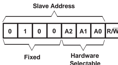
Figure 22. PCA9554 Address
