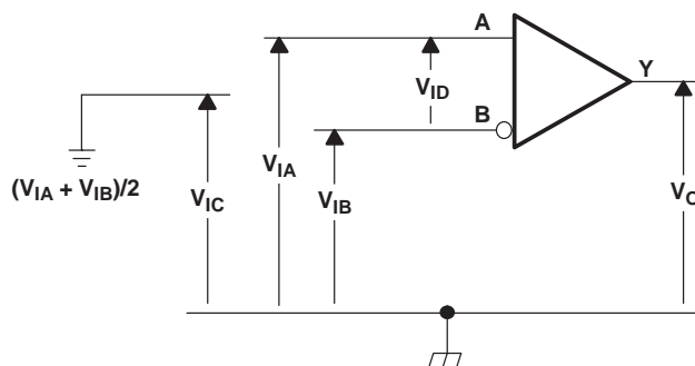
Figure 7. Voltage Definitions
