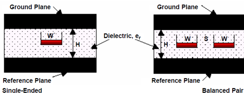
Figure 22. Stripline Topology
