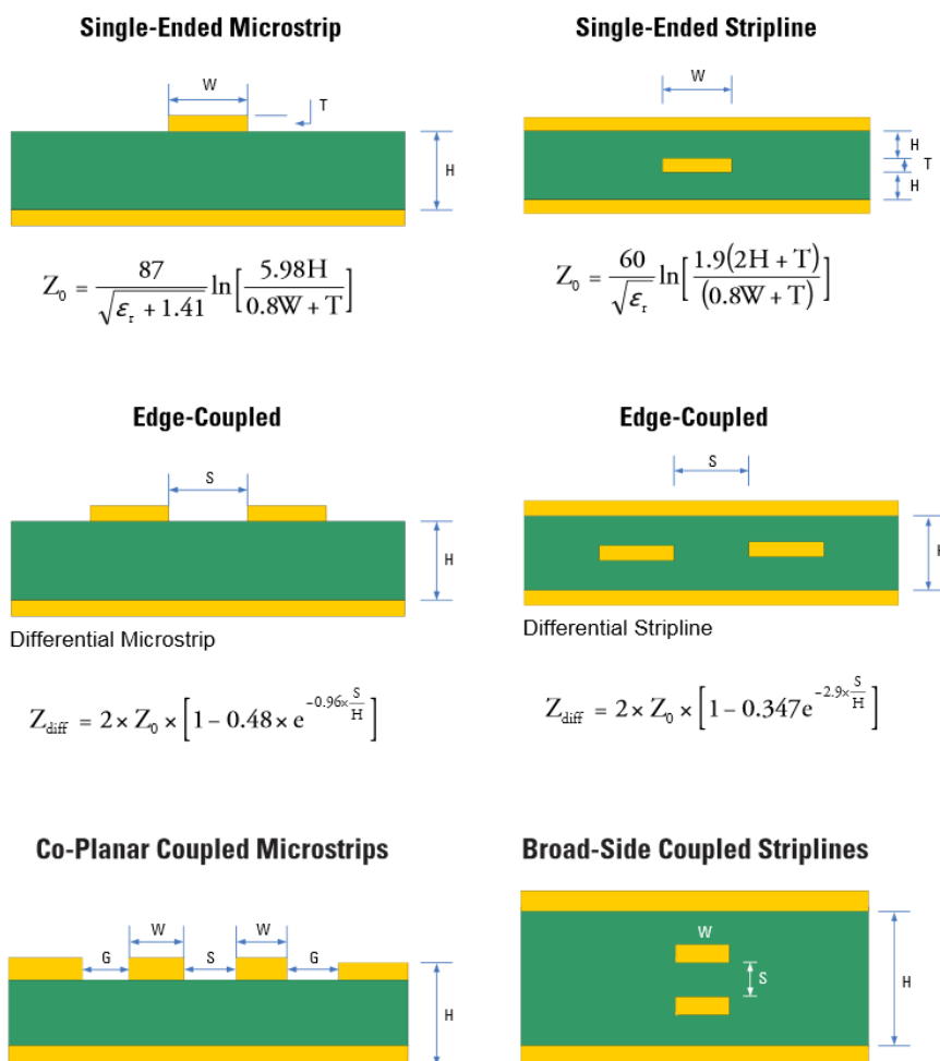
Figure 17. Controlled-Impedance Transmission Lines
