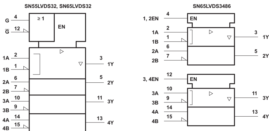
Figure 12. SN55LVDS32, SN65LVDS32, and SN65LVDS3486 Logic Symbols
