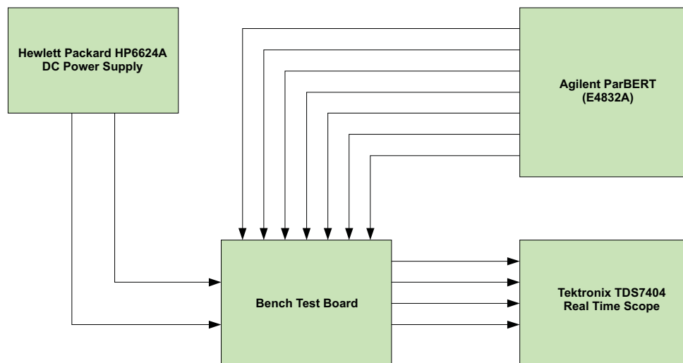
Figure 15. Equipment Setup
