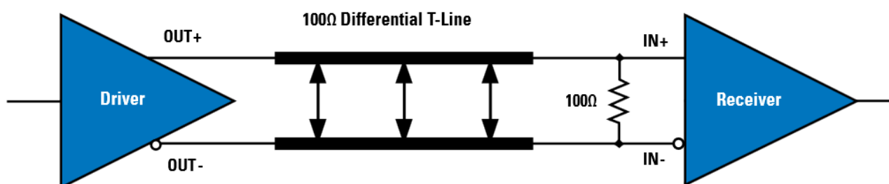
Figure 14. Point-to-Point Topology
