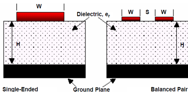
Figure 21. Microstrip Topology
