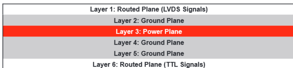
Figure 24. Six-Layer PCB Board
