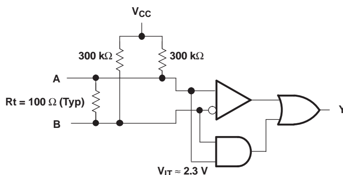
Figure 10. Open-Circuit Fail Safe of the LVDS Receiver
