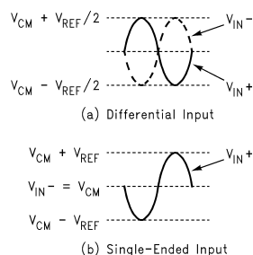
Figure 34. Expected Input Signal Range
