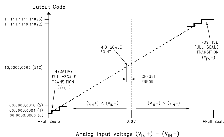
Figure 2. Transfer Characteristic
