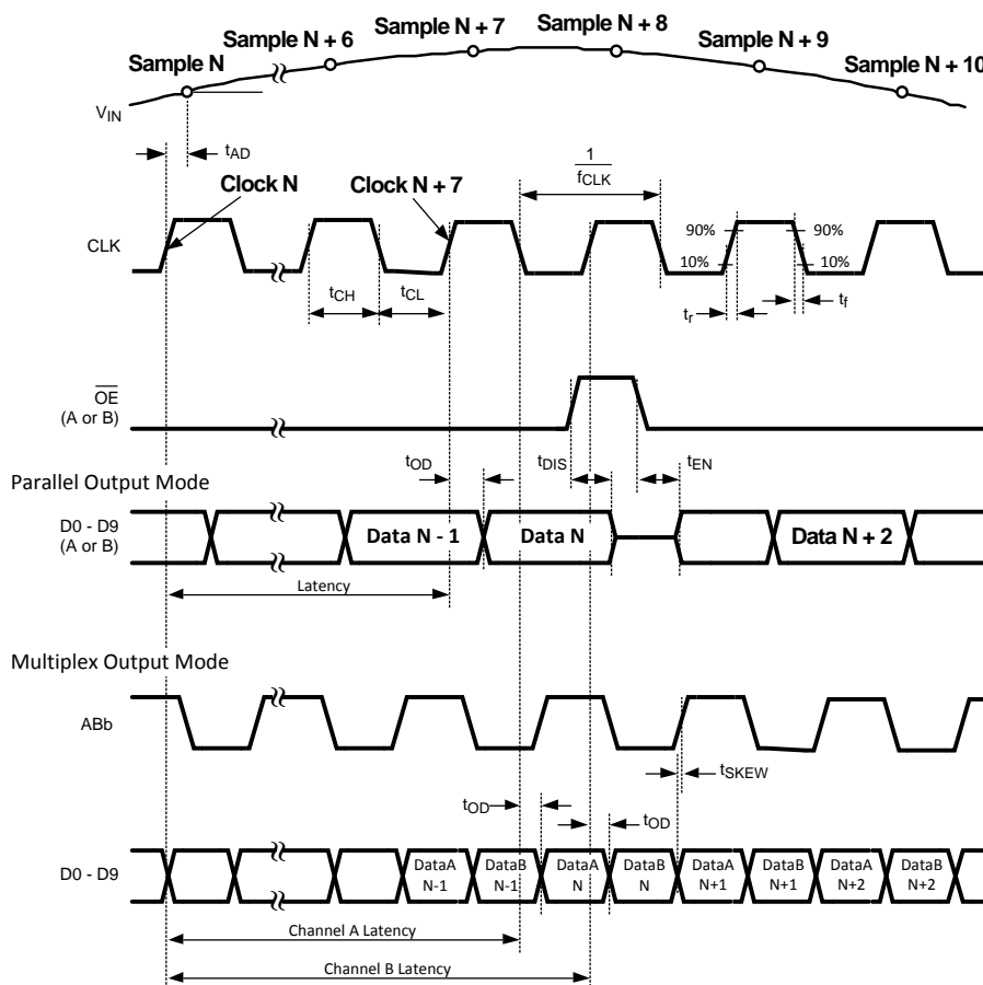
Figure 1. Output Timing
