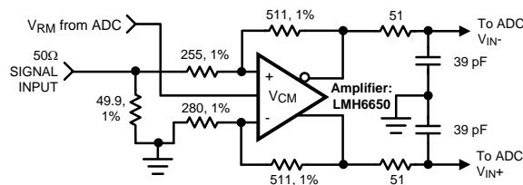
Figure 38. Optional Amplifier Differential Drive Circuit
