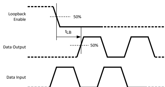
Figure 5. Loopback Delay Timing
