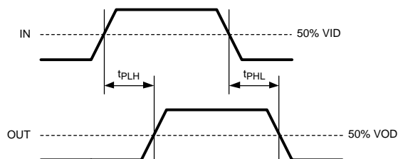
Figure 4. Propagation Delay
