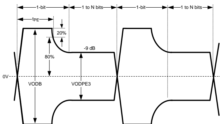
Figure 6. Output De-Emphasis Duration
