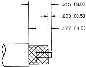
RECOMMENDED CABLE STRIPPING DIM'S
