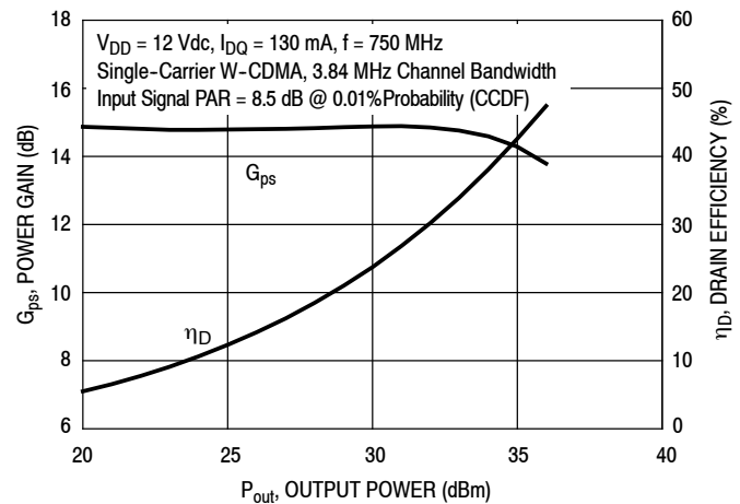
Figure 13. Single-Carrier W-CDMA Power Gain and Drain Efficiency versus Output Power
