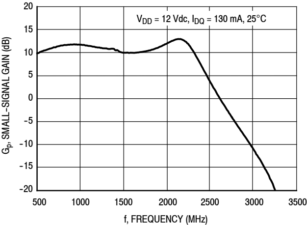
Figure 17. Small-Signal Gain versus Frequency
