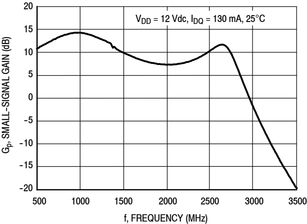
Figure 24. Small-Signal Gain versus Frequency
