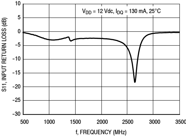
Figure 25. Input Return Loss versus Frequency
