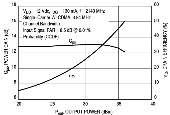
Figure 20. Single-Carrier W-CDMA Power Gain and Drain Efficiency versus Output Power
