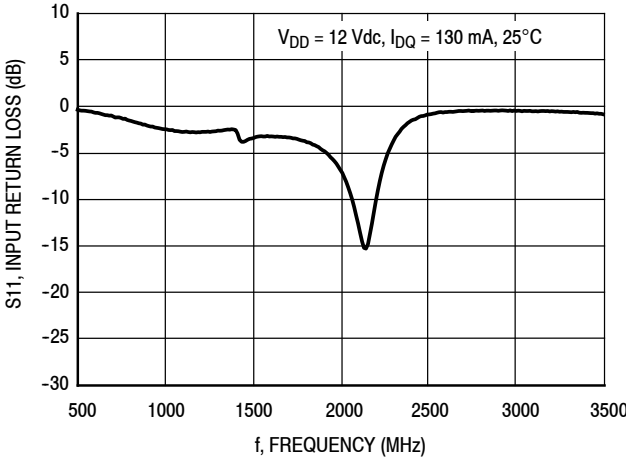
Figure 18. Input Return Loss versus Frequency
