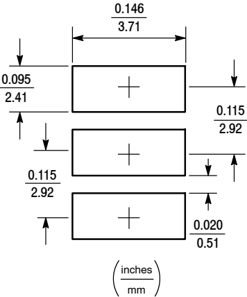
Figure 29. PLD-1.5 Solder Footprint
