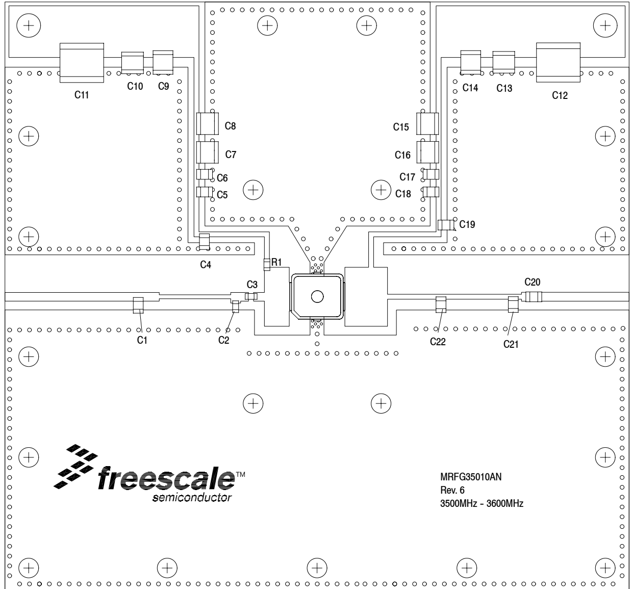
Figure 1. MRFG35010ANT1 Test Circuit Component Layout — 3550 MHz
