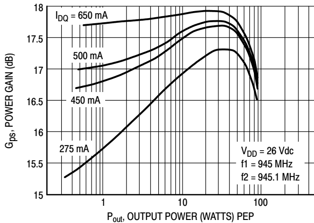
Figure 4. Power Gain versus Output Power
