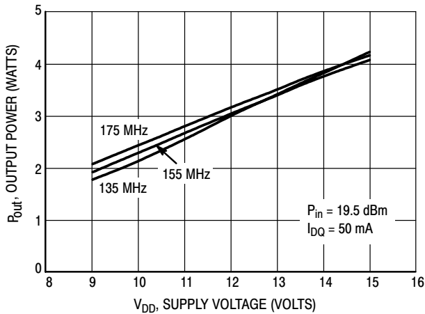
Figure 26. Output Power versus Supply Voltage
