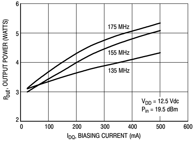
Figure 24. Output Power versus Biasing Current
