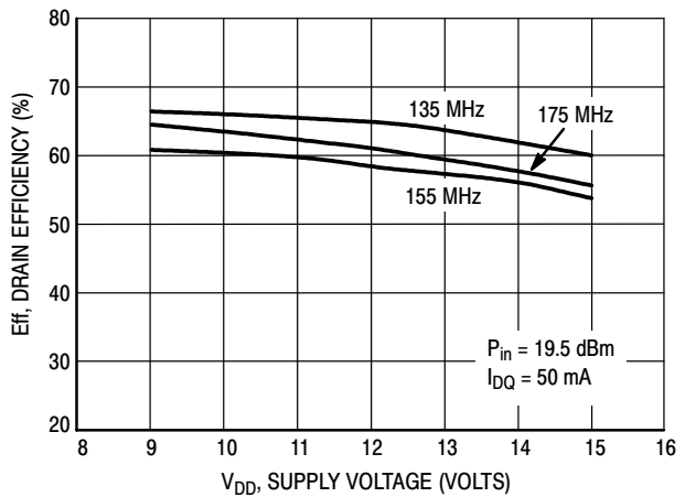
Figure 27. Drain Efficiency versus Supply Voltage
