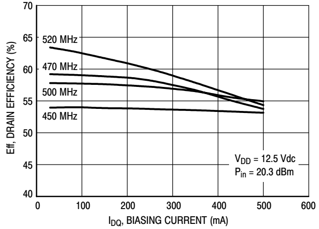
Figure 7. Drain Efficiency versus Biasing Current
