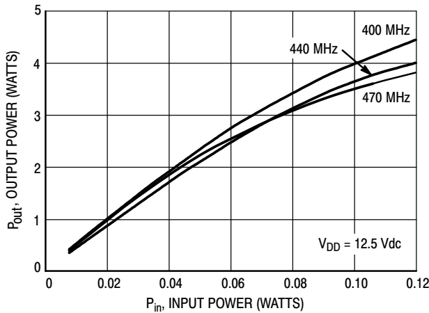
Figure 11. Output Power versus Input Power
