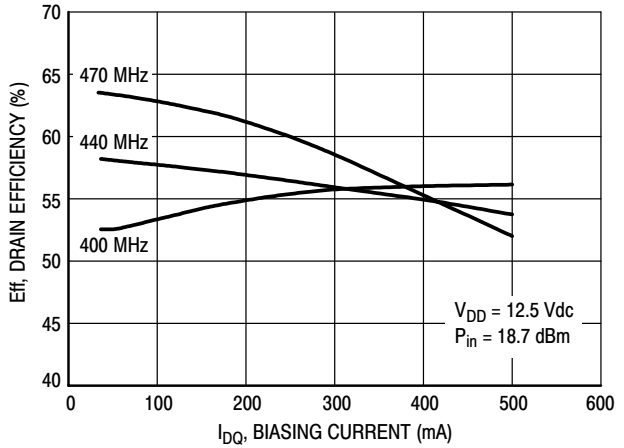
Figure 16. Drain Efficiency versus Biasing Current
