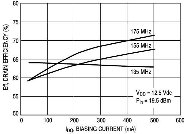
Figure 25. Drain Efficiency versus Biasing Current
