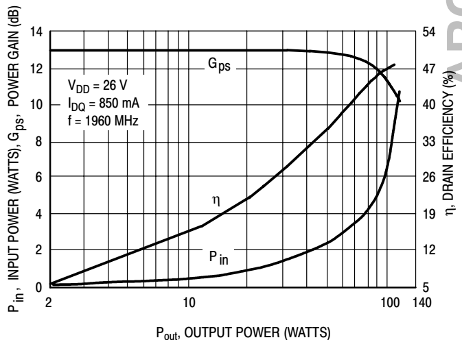
Figure 8. CW Performance
