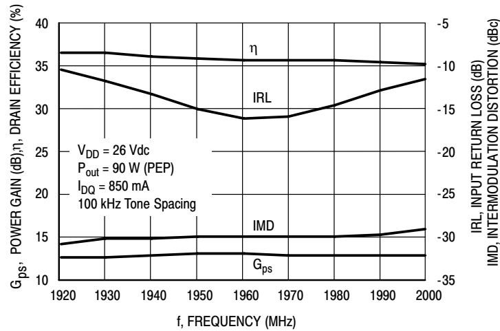
Figure 11. Two-Tone Broadband Performance
