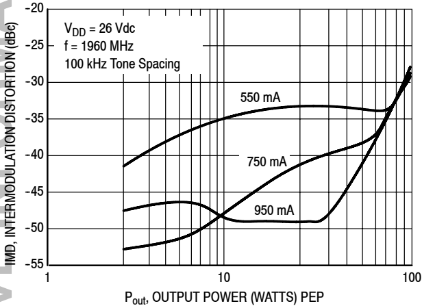
Figure 5. Third Order Intermodulation Distortion versus Output Power
