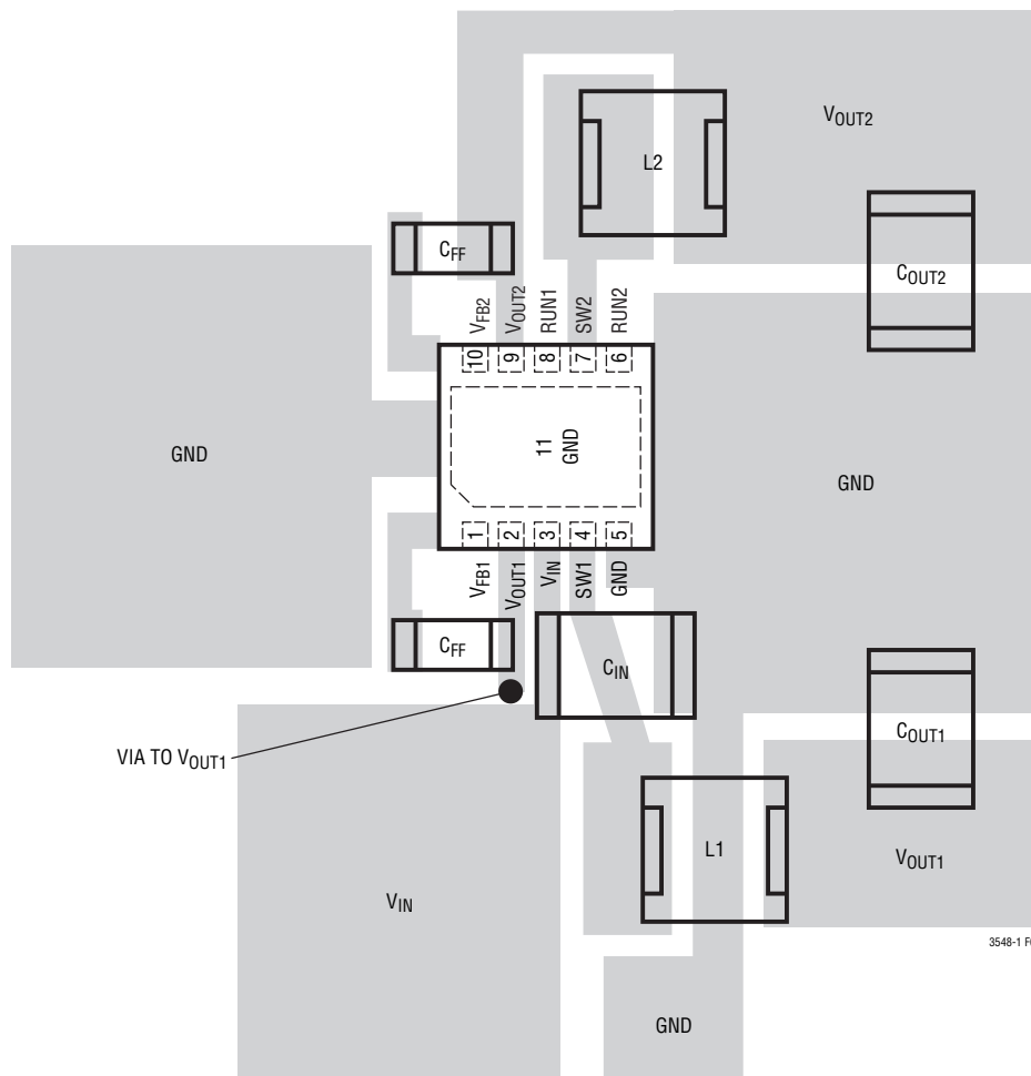
Figure 4. LTC3548-1 Layout Diagram
