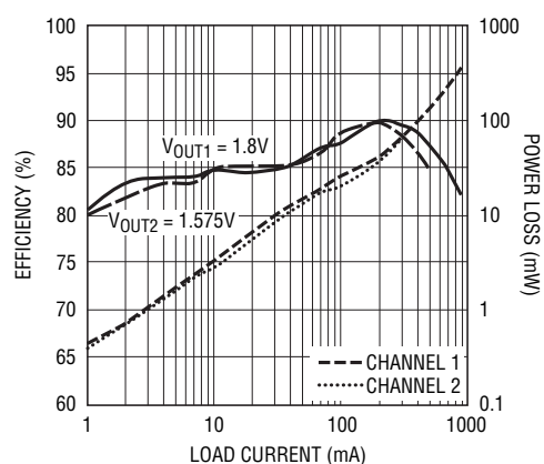
LTC3548-1 Efficiency Curve/Power Loss
