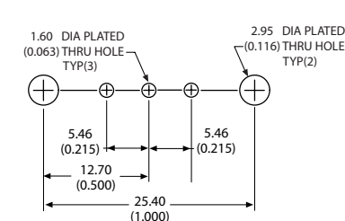
Recommended hole pattern for 8241-CL11G
