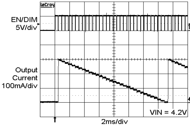
Figure 21. Enable and Output Current Dimming Waveforms
