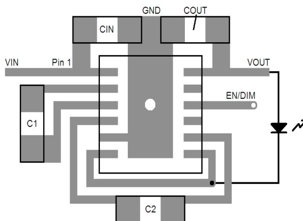
Figure 29. Recommended Layout
