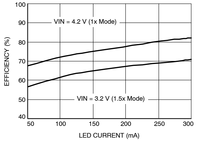
Figure 4. Efficiency vs. LED Current
