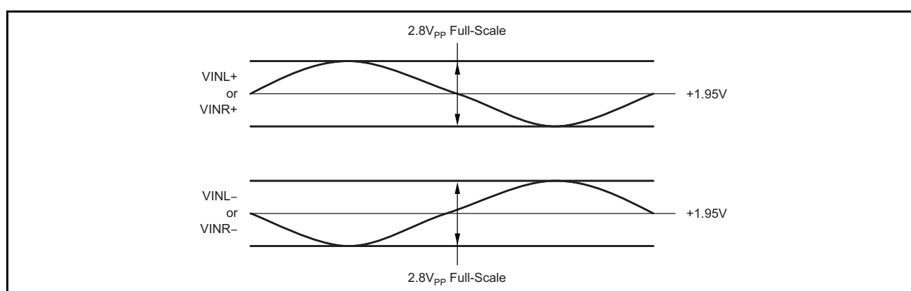
Figure 35. Full-Scale Analog Input Range
