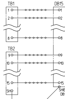
TYPICAL SCHEMATIC (15 POSITION SHOWN)
