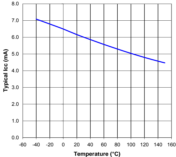
Icc vs Temperature
