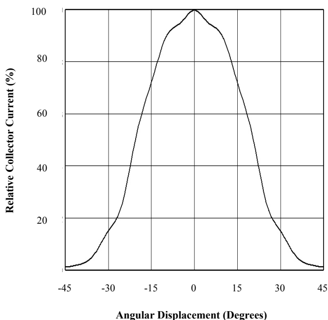
OP552 - Angular Response
