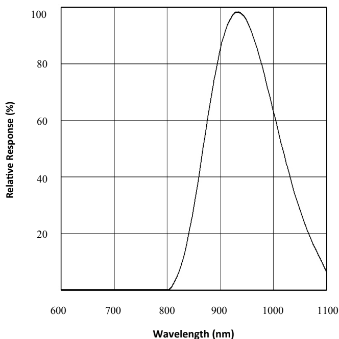
OP552 - Typical Spectral Response
