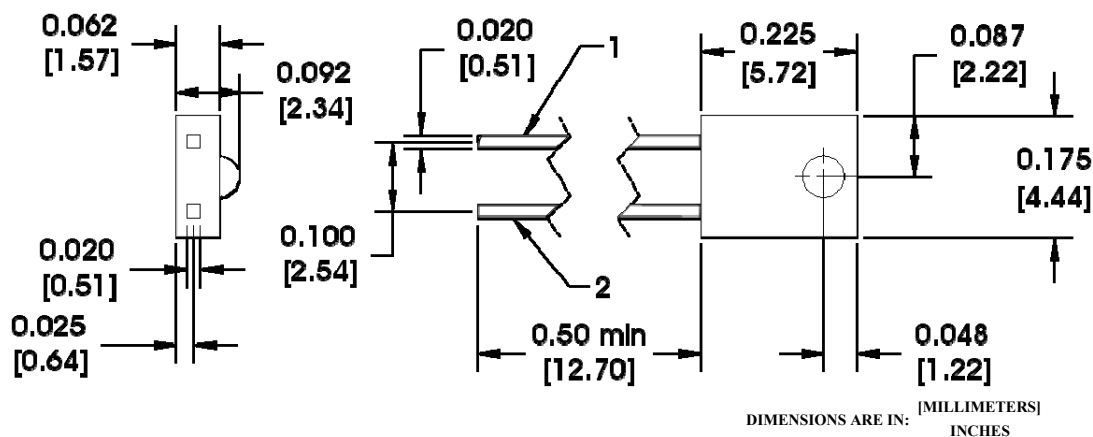
OP555, OP565, OP755, OP775 (A, B, C, D)
