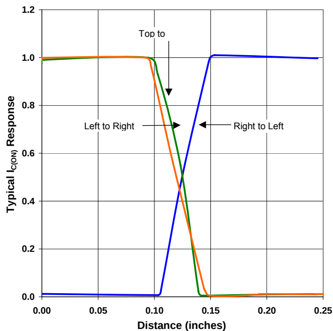
OPB885 - Flag Next to Sensor
