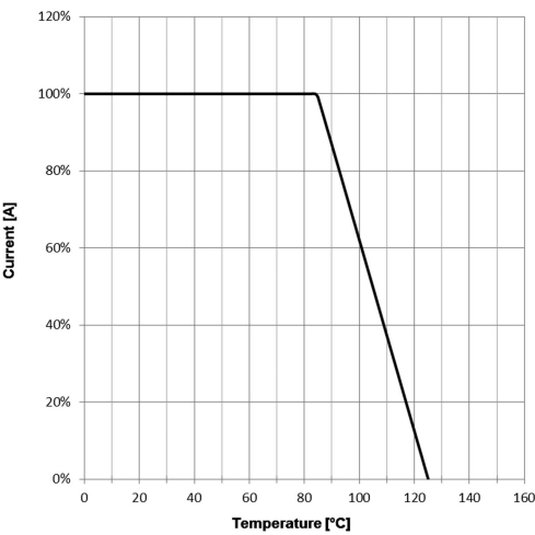
F2 Derating Curve:
