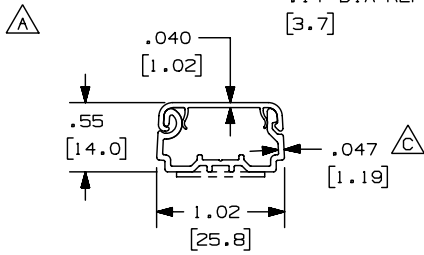
LDPH5 CLOSED POSITION
