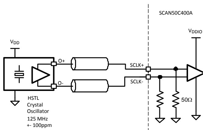
Figure 2. SCLK_{\pm} Driven by HSTL Clock Driver / Crystals
