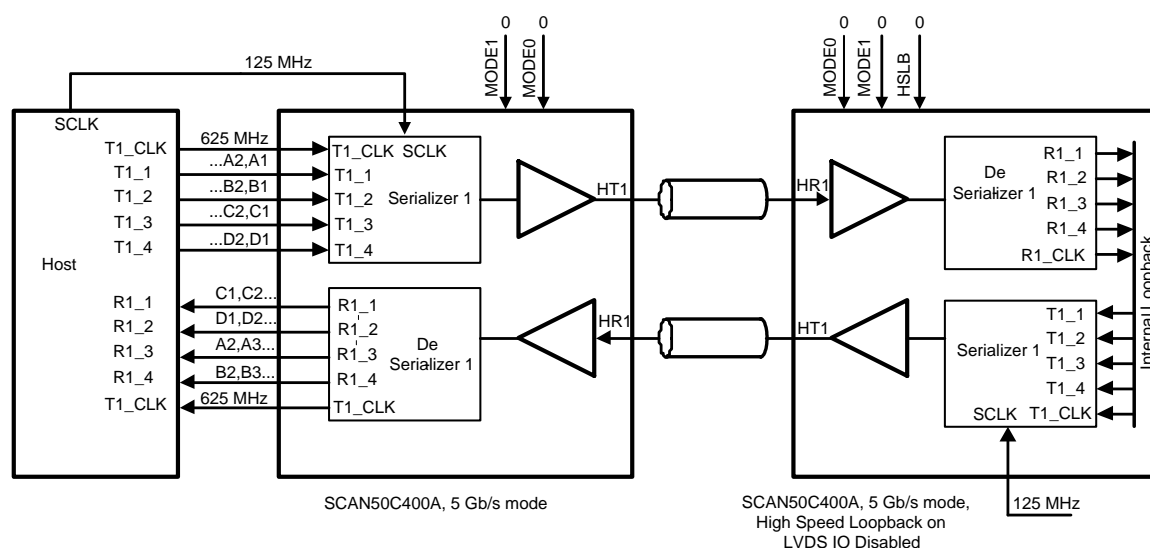
Figure 8. SCAN50C400A in High-Speed Loopback (5 Gbps Shown)
