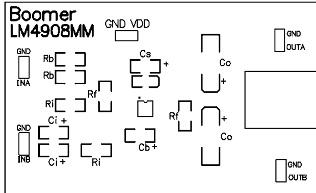
Figure 47. Recommended VSSOP Board Layout: Top Overlay
