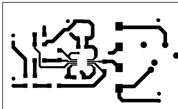
Figure 48. Recommended VSSOP Board Layout: Top Layer
