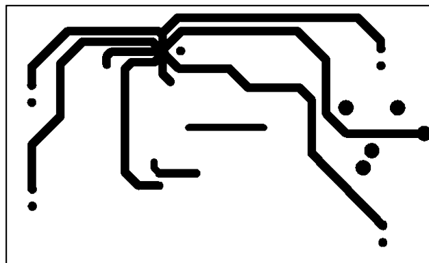
Figure 49. Recommended VSSOP Board Layout: Bottom Layer
