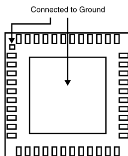
Figure 4. WQFN Package Bottom View
