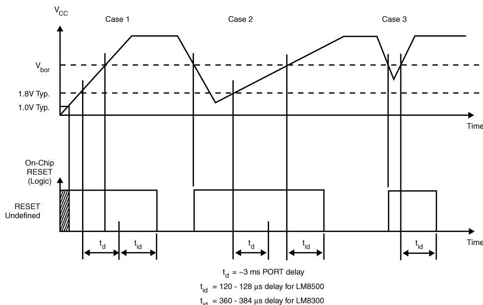
Figure 7. Brownout Reset Operation
