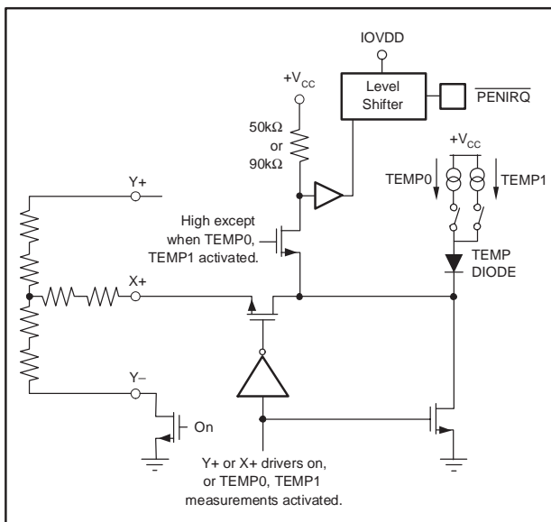
Figure 10. \overline{\text{PENIRQ}} Functional Block Diagram
