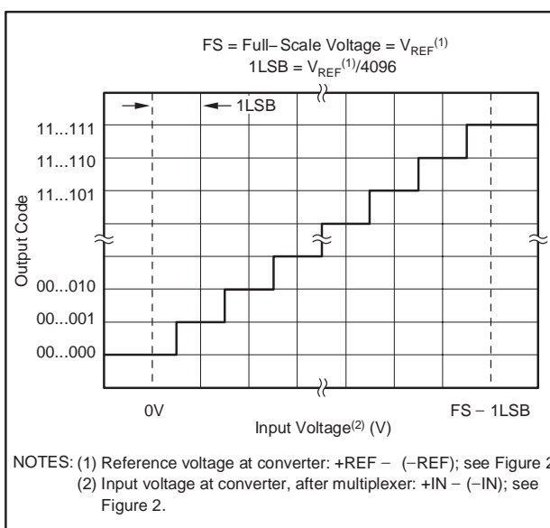
Figure 14. Ideal Input Voltages and Output Codes
