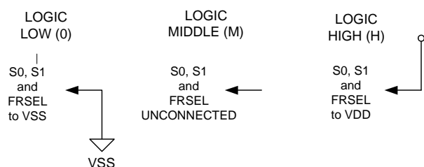
Figure 2. 3-Level Logic
