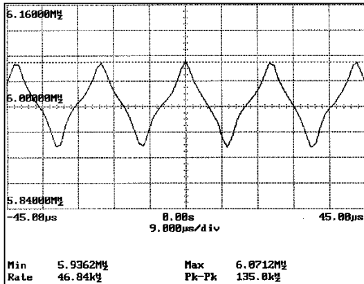
Figure 4. Spread Spectrum Profiles (Frequency versus Time)
