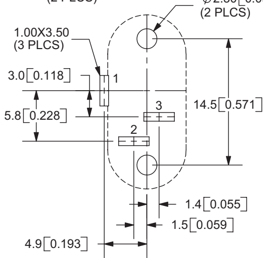
PCB LAYOUT FRONT VIEW
