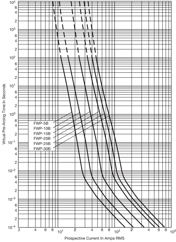
Time-Current Curve
