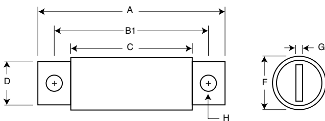
Fig. 2: 35-400A
