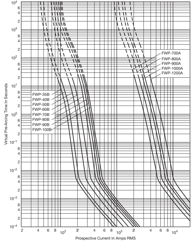
Time-Current Curve
