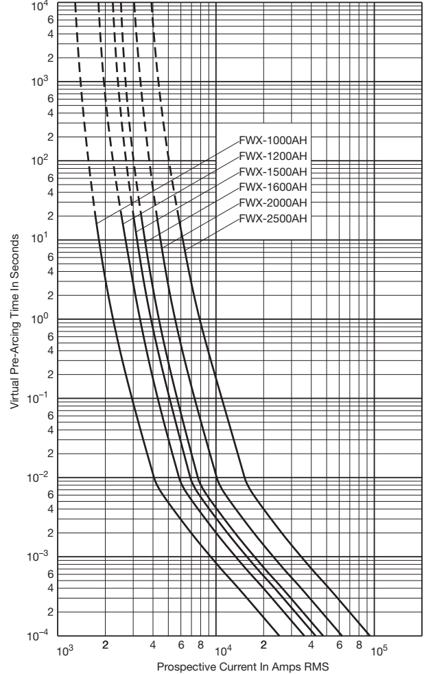
Time-Current Curve
