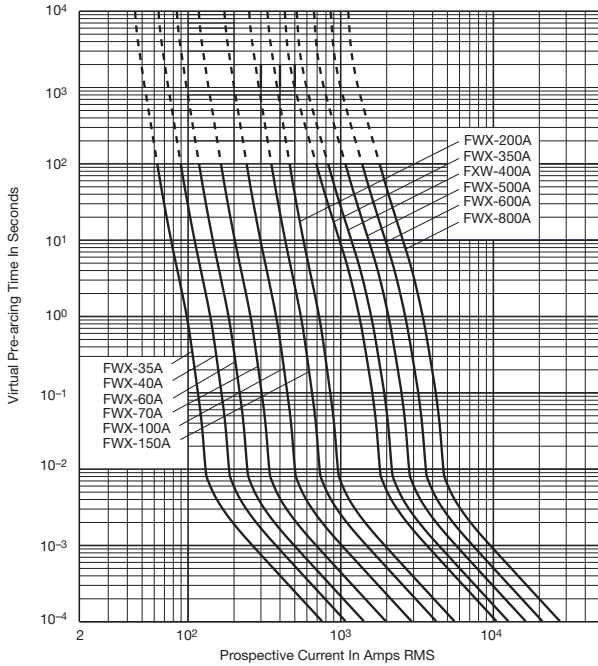
Time-Current Curve
