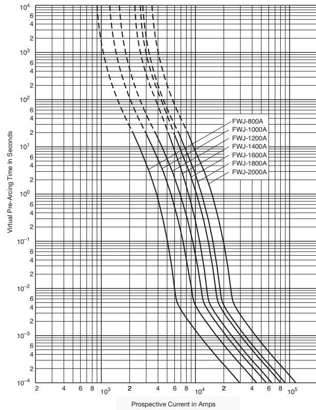
Time-Current Curve
