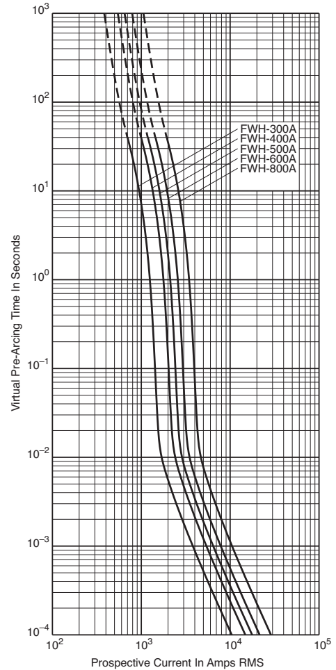
Time-Current Curve
