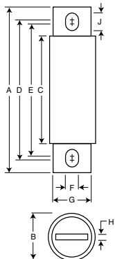
Fig. 1: 5-800A
