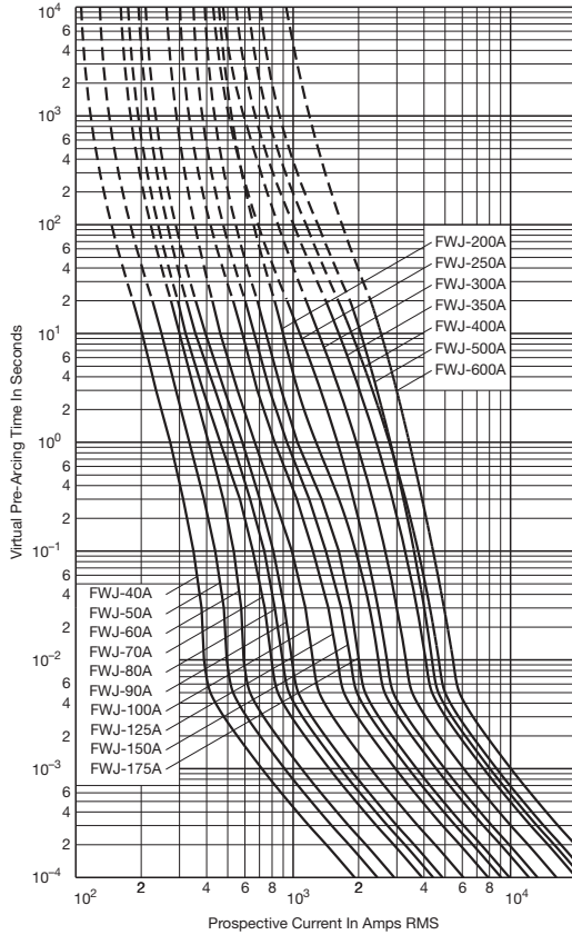
Time-Current Curve
