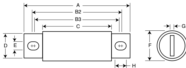
Fig. 2: 35-400A
