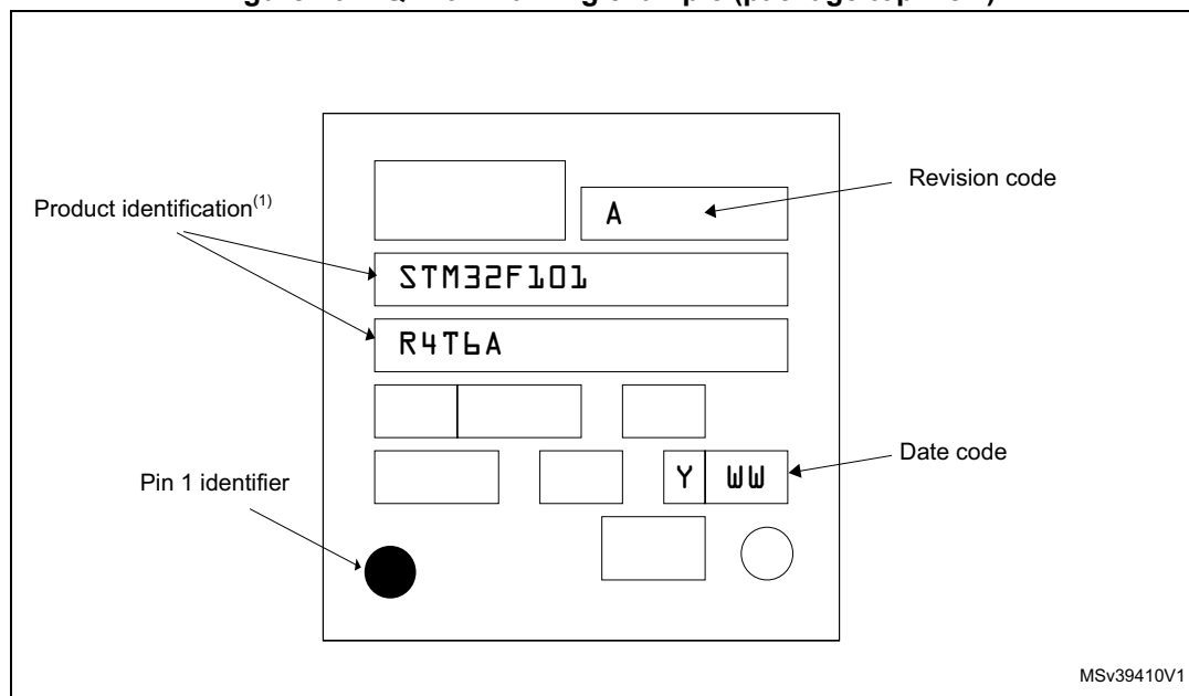
Figure 40. LQFP64 marking example (package top view)
