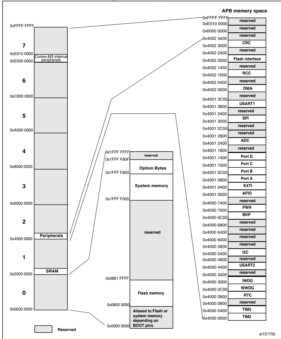
Figure 7. Memory map
