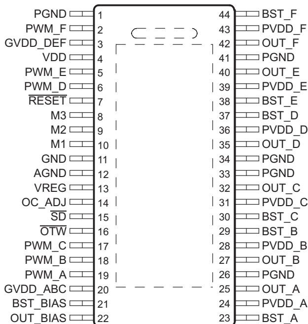
DDW PACKAGE (TOP VIEW)
