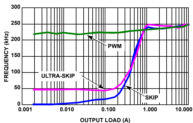
FIGURE 5. V_{OUT2} = 1.05V FREQUENCY vs LOAD
