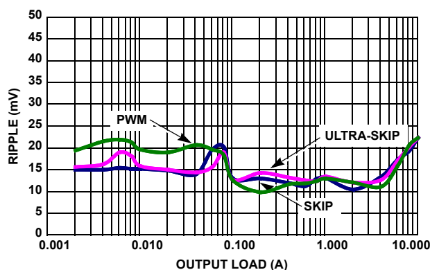
FIGURE 6. V_{OUT2} = 1.05V RIPPLE vs LOAD
