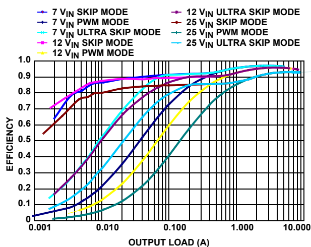
FIGURE 4. V_{OUT1} = 5V EFFICIENCY vs LOAD (400kHz)
