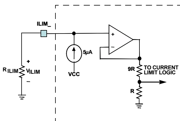
FIGURE 25. CURRENT LIMIT BLOCK DIAGRAM
