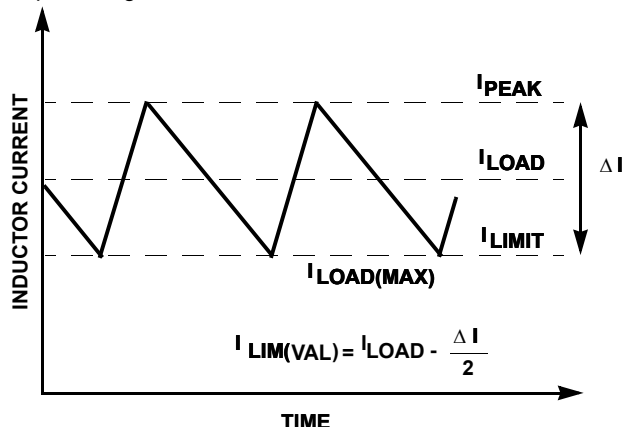
FIGURE 24. "VALLEY" CURRENT LIMIT THRESHOLD POINT
