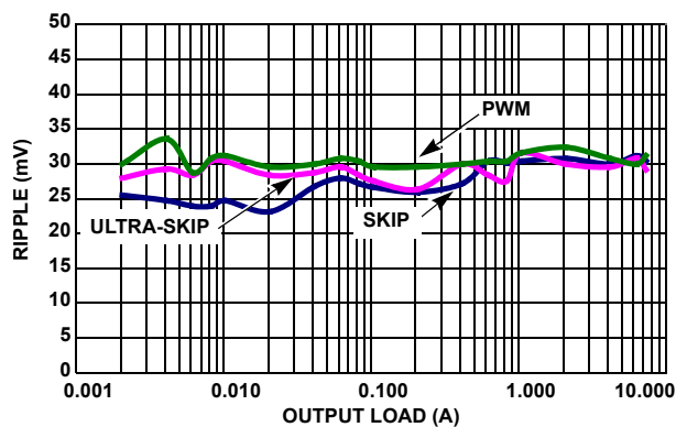
FIGURE 8. V_{OUT1} = 1.5V RIPPLE vs LOAD
