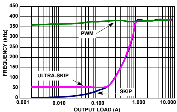
FIGURE 11. V_{OUT1} = 5V FREQUENCY vs LOAD
