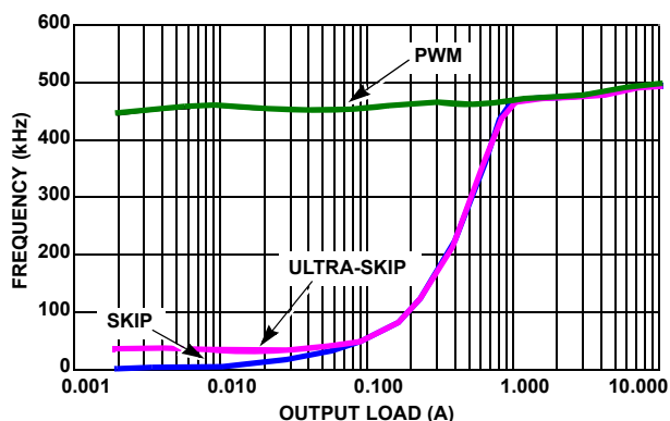
FIGURE 9. V_{OUT2} = 3.3V FREQUENCY vs LOAD
