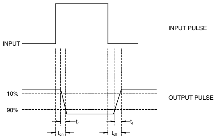
Waveforms
