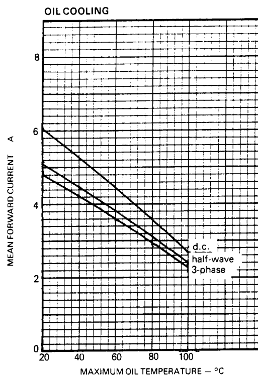
DERATING CURVES
