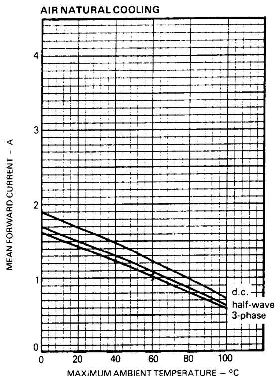
DERATING CURVES
