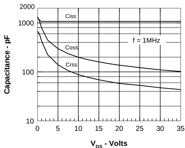
Figure 8. Capacitance Curves
