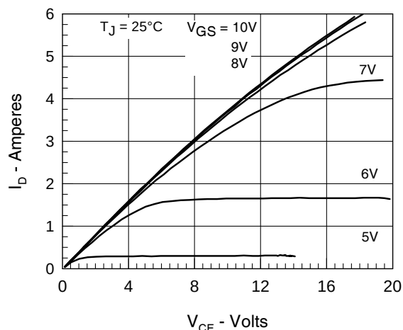
Figure 2. Extended Output Characteristics at 125°C
