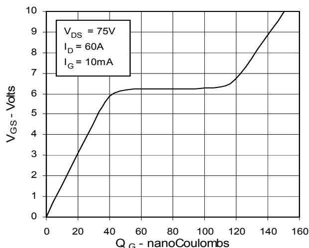
Fig. 10. Gate Charge
