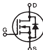
TO-247 (IXFH)
